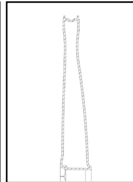
CROSS SECTION FFWD FALCON
